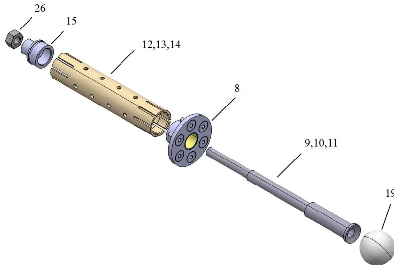
Fig. 3: Thermal expansion compensator.
