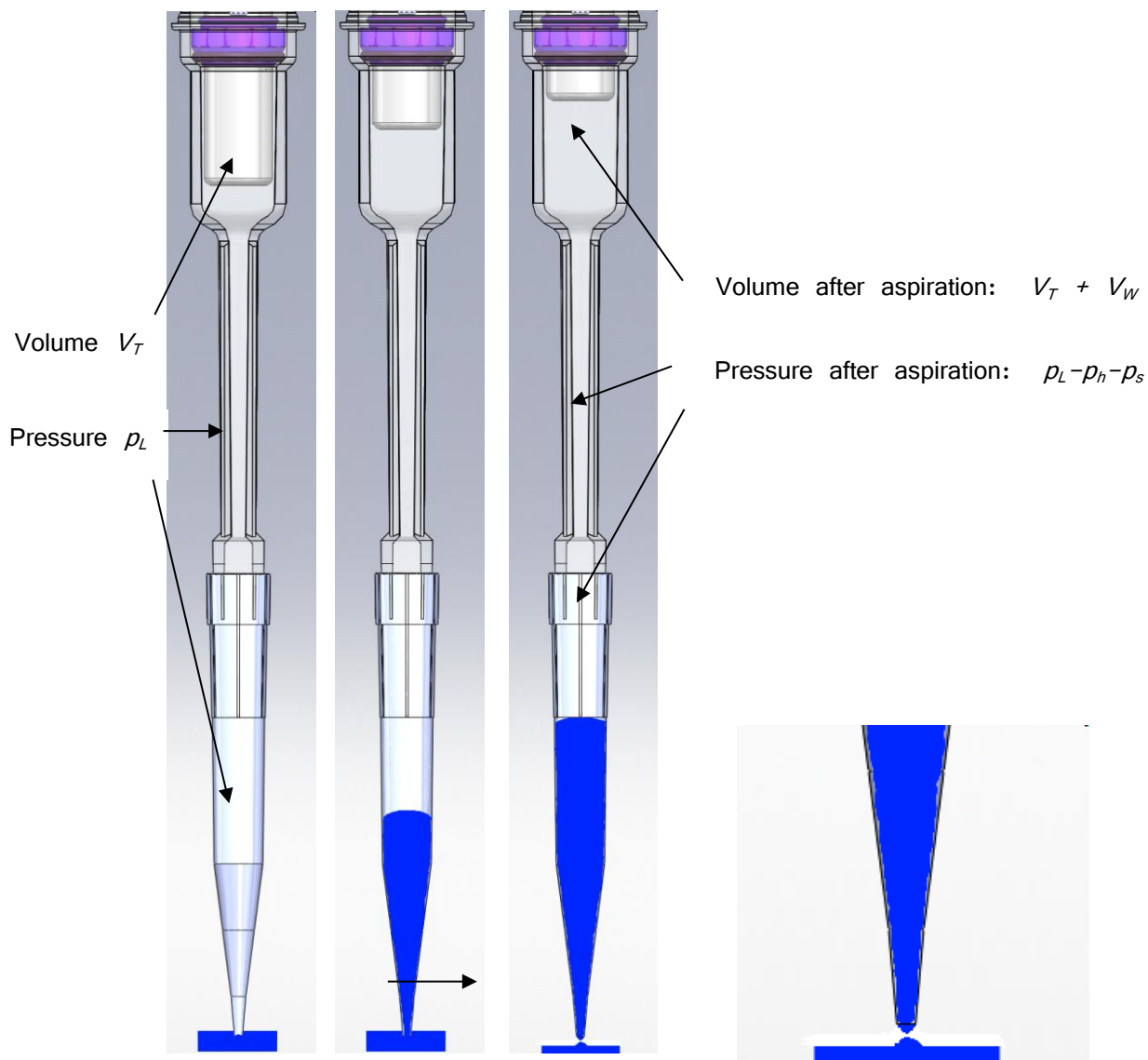
Figure 1: Aspiration of liquid in the pipette
