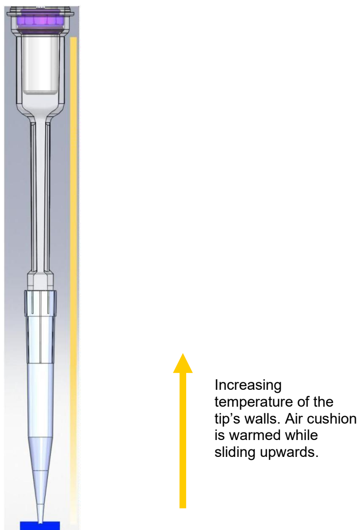
Figure 2: Pipetting of cold liquid
