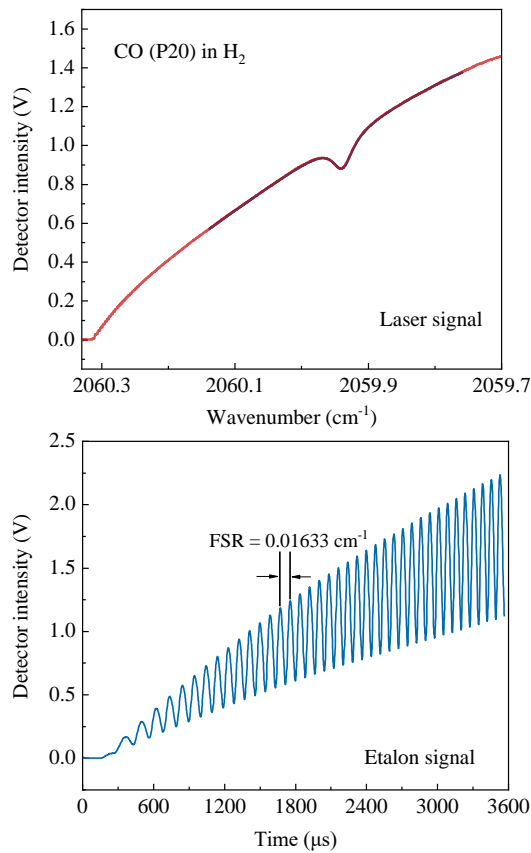
Figure 3. Raw data of laser signal and etalon signal measured in the gas cell
