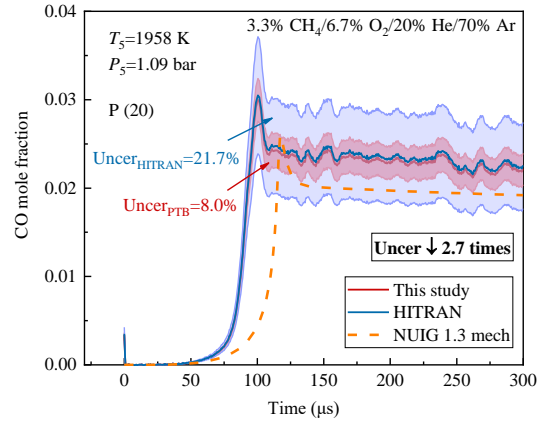
Figure 12. Time-resolved CO mole fraction of CH 4 oxidation measured in the shock tube and calculated using NUIG 1.3 mechanism 40
