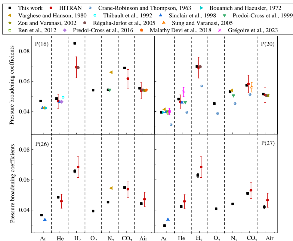
Figure 6. Comparison of pressure broadening coefficients with literature results (the error bars are hidden within the symbol)
