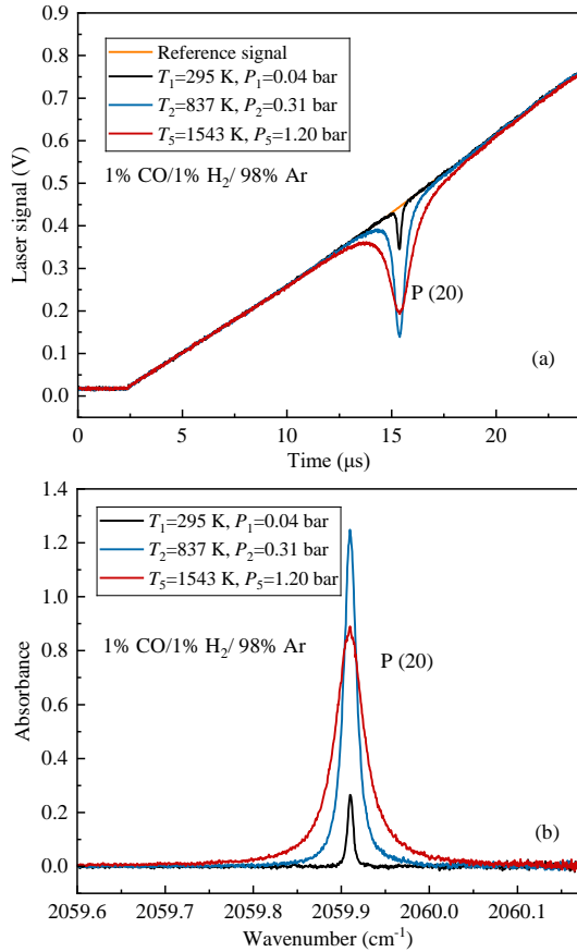
Figure 8. Laser signal (a) and measured spectra (b) of CO at different status in the shock tube
