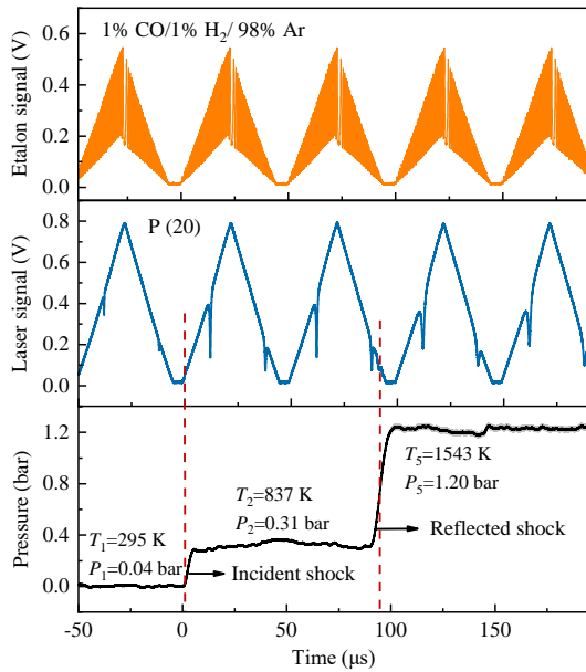
Figure 7. Raw data of laser signal, etalon signal, and pressure measured in the shock tube
