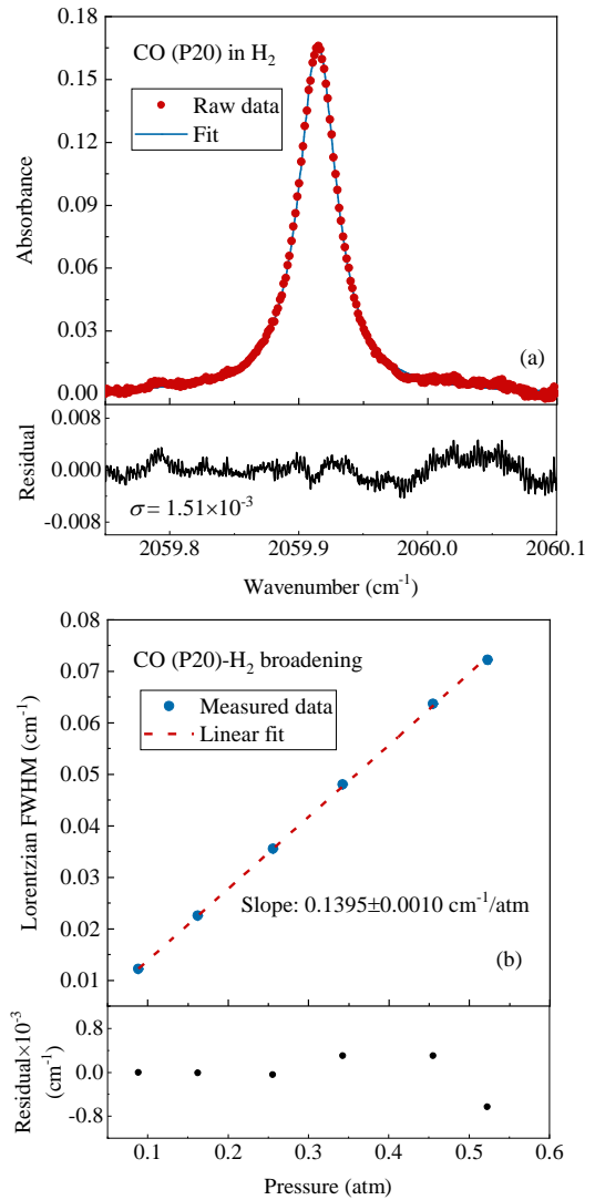
Figure 4. (a) CO absorption spectrum of P(20) in \text{H}_2 ; (b) CO- \text{H}_2 pressure broadening of P(20) (the x and y axis error bars are hidden within the symbol)
