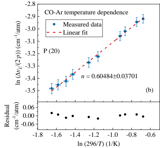
Figure 9. (a) CO absorption spectra in 1% CO/1% H 2 /98% Ar; (b) Temperature dependence coefficient of CO-Ar
