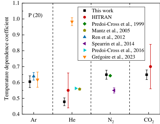
Figure 11. Comparison of temperature dependency coefficients with literature results
