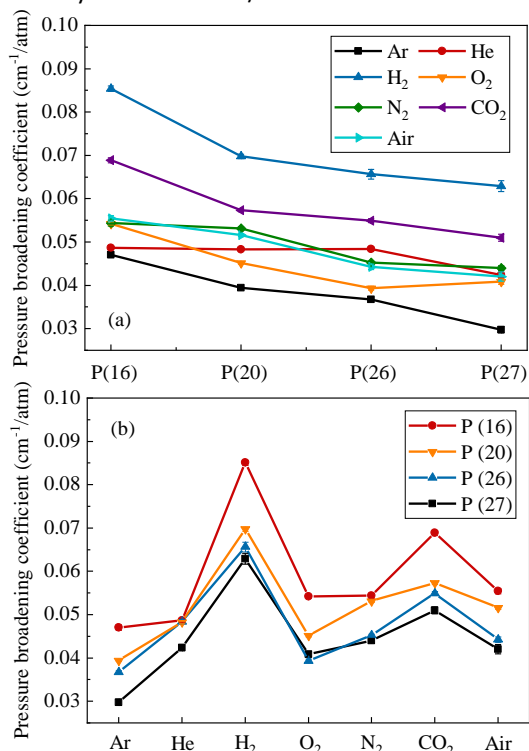
Figure 5. (a) Pressure broadening coefficients versus line numbers; (b) Pressure broadening coefficients versus buffer gases (the error bars are hidden within the symbol)
