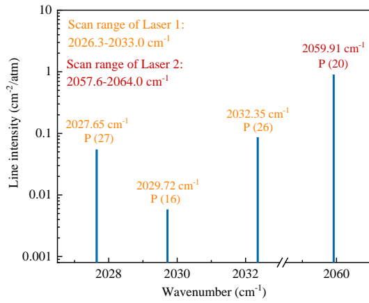
Figure 2. CO transitions measured in this study
