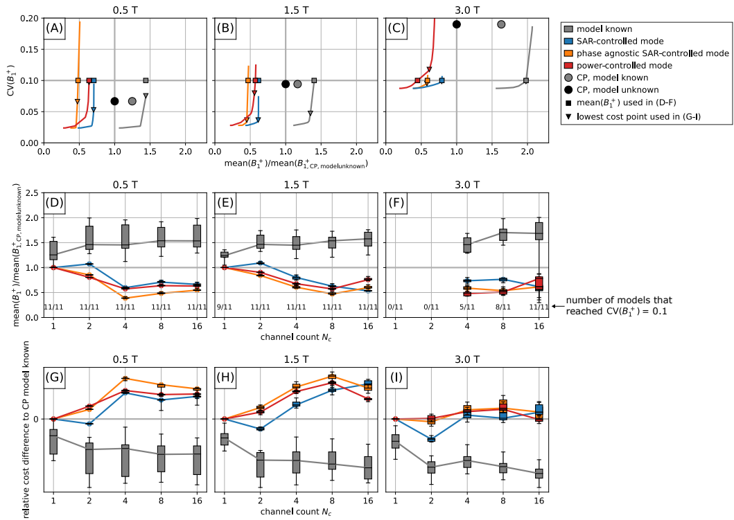
Fig. A.5: \text{mean}(B_1^+) performance for SCM, PASC and PCM (the limits of all 11 models under test with an additional safety factor are considered each) or with model known (SCM, limits of current model only, no safety factor). \text{mean}(B_1^+) is plotted relative to the \text{mean}(B_1^+) of the CP mode with unknown model condition (combined limits of all 11 models with additional safety factor). (A-C) Trade-off between \text{mean}(B_1^+) and \text{CV}(B_1^+) for model Duke and 8 channels. (D-F) \text{mean}(B_1^+) that reaches \text{CV}(B_1^+) = 0.1 divided by the \text{mean}(B_1^+) of the CP mode. Higher values are better. (G-I) Difference of cost C = -\text{mean}(B_1^+)/\mu T + 3 \times \text{CV}(B_1^+) between CP mode and the best shim vector of pTx optimised shim vectors. G-I use different y-scales and are hence not directly comparable.
