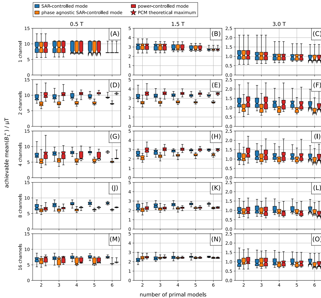
Fig. 4.19: Maximum \text{mean}(B_1^+) in all evaluation models as function of primal model count for all possible combinations of evaluation and primal models. Safety limits are derived from the primal models in an anchor-target analysis with the leave one out method to obtain a safety factor. The 10^6 random RF-shim vectors are subsequently used to calculate the maximum \text{mean}(B_1^+) in the previously unseen evaluation models.
