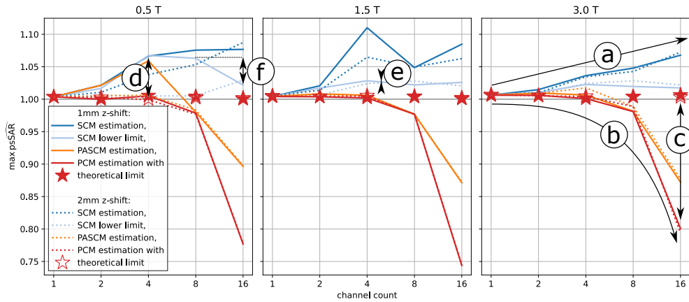
Fig. 4.4: Maximum \widehat{\text{psSAR}} in model Duke for an anchor-target analysis with z-shifts of 1 mm and 2 mm. Features (a-f) are explained in the text. This figure by Petzold et al. [91] is licenced under CC BY 4.0.
