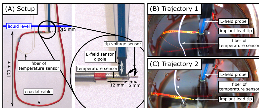
Fig. 6.1: Experimental setup to correlate implant tip heating with E-field and tip temperature. (A) A semi-rigid coaxial cable with uninsulated tip is bent into a loop. A fibre-optical temperature sensor is attached to the tip. An E-field sensor is positioned to be close to the tip (see zoom). (B) Trajectory 1 in the PVP/water phantom and 8-channel head coil. (C) Trajectory 2 where the tip was bent approximately 50 mm. This figure by Petzold et al. [35] is licenced under CC BY 4.0 and was adapted by rearranging the panels.
