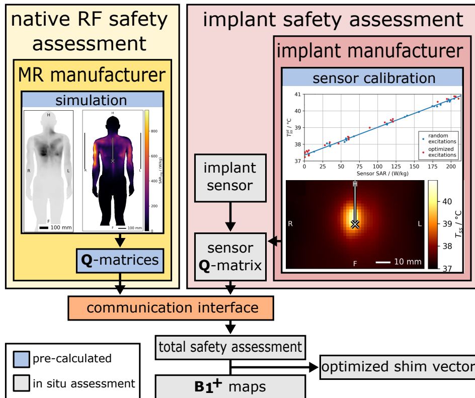
Fig. 1.1: Diagram of the proposed safety concept for AIMDs. The MR system manufacturer is responsible to provide pTx safety limits for patients without implant (native case, left). The implant manufacturer is responsible to provide calibrated sensor information about the implant hazard. With this prior information, a patient and situation specific sensor Q-matrix can be acquired from a short sequence of low-power measurements with the patient in the scanner. Optimised RF-shim vectors can be obtained by combining native and implant Q-matrices with the channel-wise B_1^+ maps. This figure by Petzold et al. [35] is licenced under a creative commons attribution 4.0 international licence that can be found under https://creativecommons.org/licenses/by/4.0/ (CC BY 4.0).
