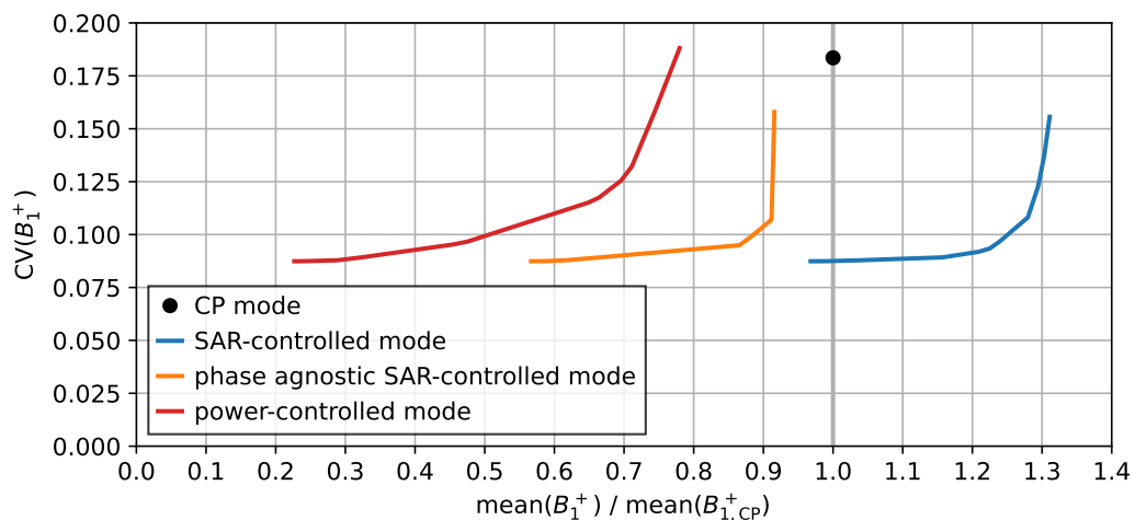
Fig. 4.1: Trade-off between optimised \text{mean}(B_1^+) and \text{CV}(B_1^+) of all three safety limits SCM, PASC and PCM for model Duke at 3 T and 8 channels in cardiac imaging position.
