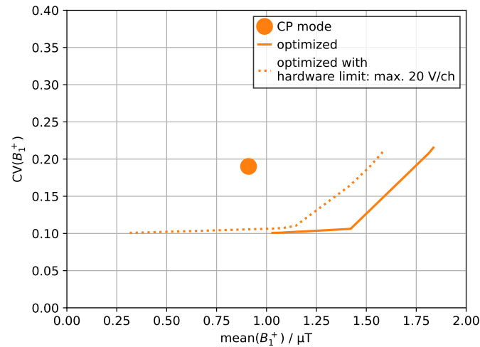
Fig. 5.11: (A) Trade-off between CV(B_1^+) and \text{mean}(B_1^+) for SCM, implant tip limit \text{SAR}_{10\text{g}} \leq 10 \text{ W kg}^{-1} and with additional hardware limit u_c \leq 20 . This figure by Petzold et al. [35] is licenced under CC BY 4.0 and was adapted by using a different hardware limit.
