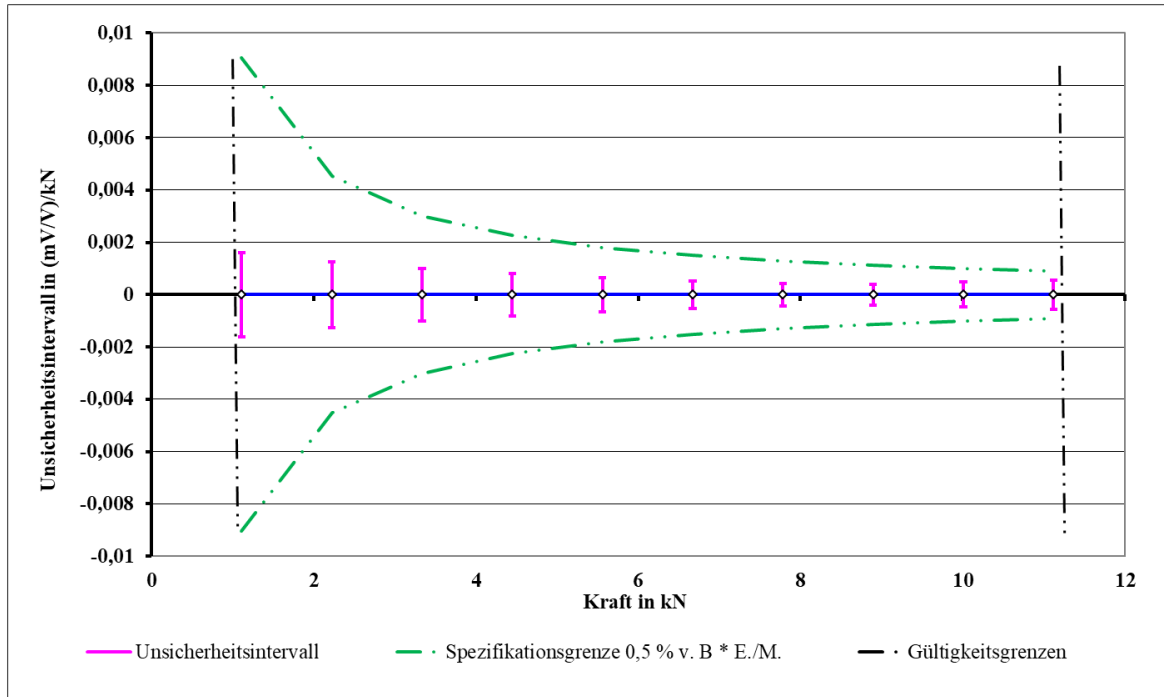
Figure 16: as in Figure 14, but with hyperbolic specification limit
