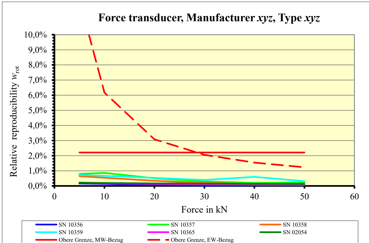
Figure 17: Visualisation of the measurement uncertainty contribution of the reproducibility
