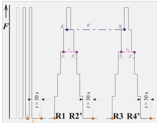
Figure 5: Example calibration sequence B; one mounting position, five force steps (2 or 3 preloads, reading after start of force change)
