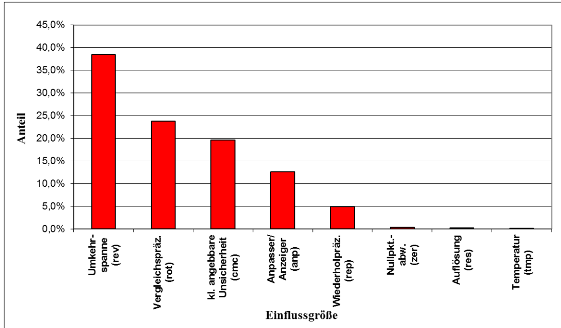
Figure 12: Example for visualising the variance components (square of the uncertainty contributions) of the total variance (square of the standard measurement uncertainty) in descending order
