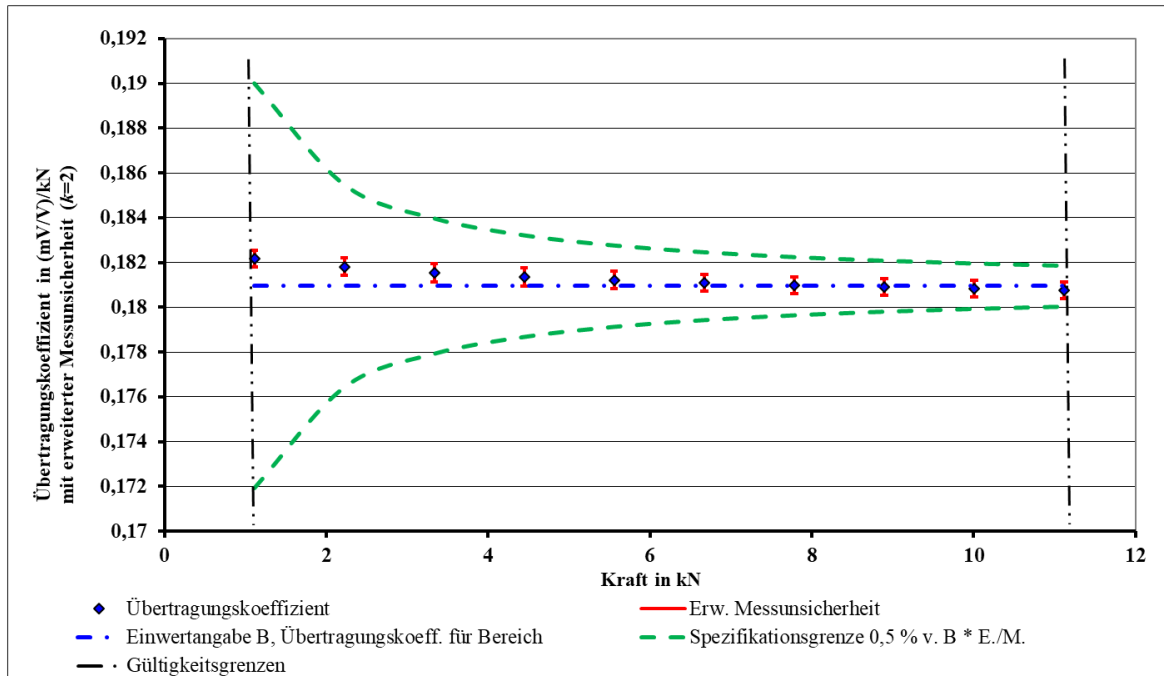
Figure 15: as in Figure 13, but with hyperbolic specification limit (B = single-figure indication; E. = calibration range end value; M. = set value)
