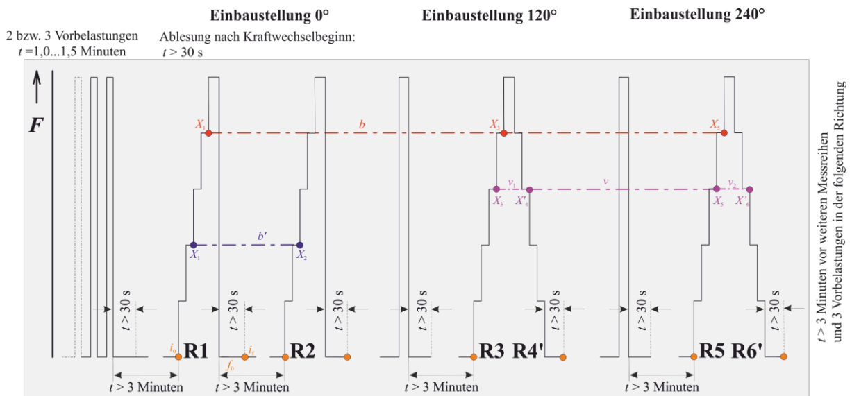
Figure 4: Example calibration sequence A; three mounting positions, five force steps (Mounting positions at 0°, 120° and 240°, 2 or 3 preloads, reading after start of force change; more than 3 minutes before further measurement series and 3 preloads in the following direction)
