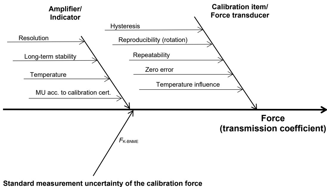
Figure 10: Influence quantities in the determination of the measurement uncertainties attributed to the transmission coefficients of a force transducer
