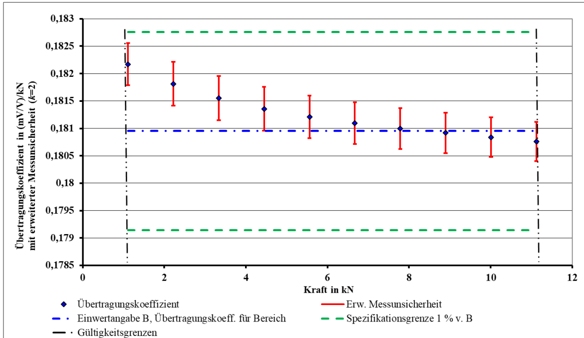
Figure 13: Transmission coefficients with expanded measurement uncertainty, single-figure indication (transmission coefficient for the range) and specification limit
