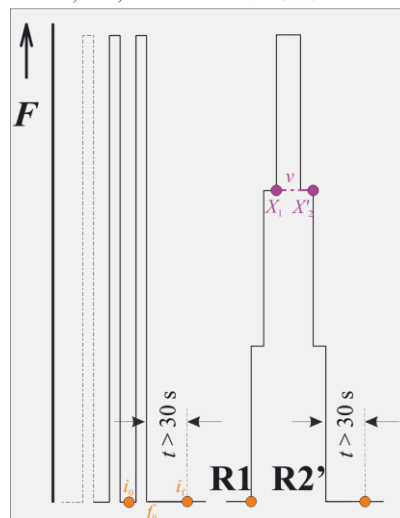
Figure 6: Example calibration sequence C; one mounting position, one measuring series, increasing and decreasing load, three force steps (2 or 3 preloads, reading after start of force change)
