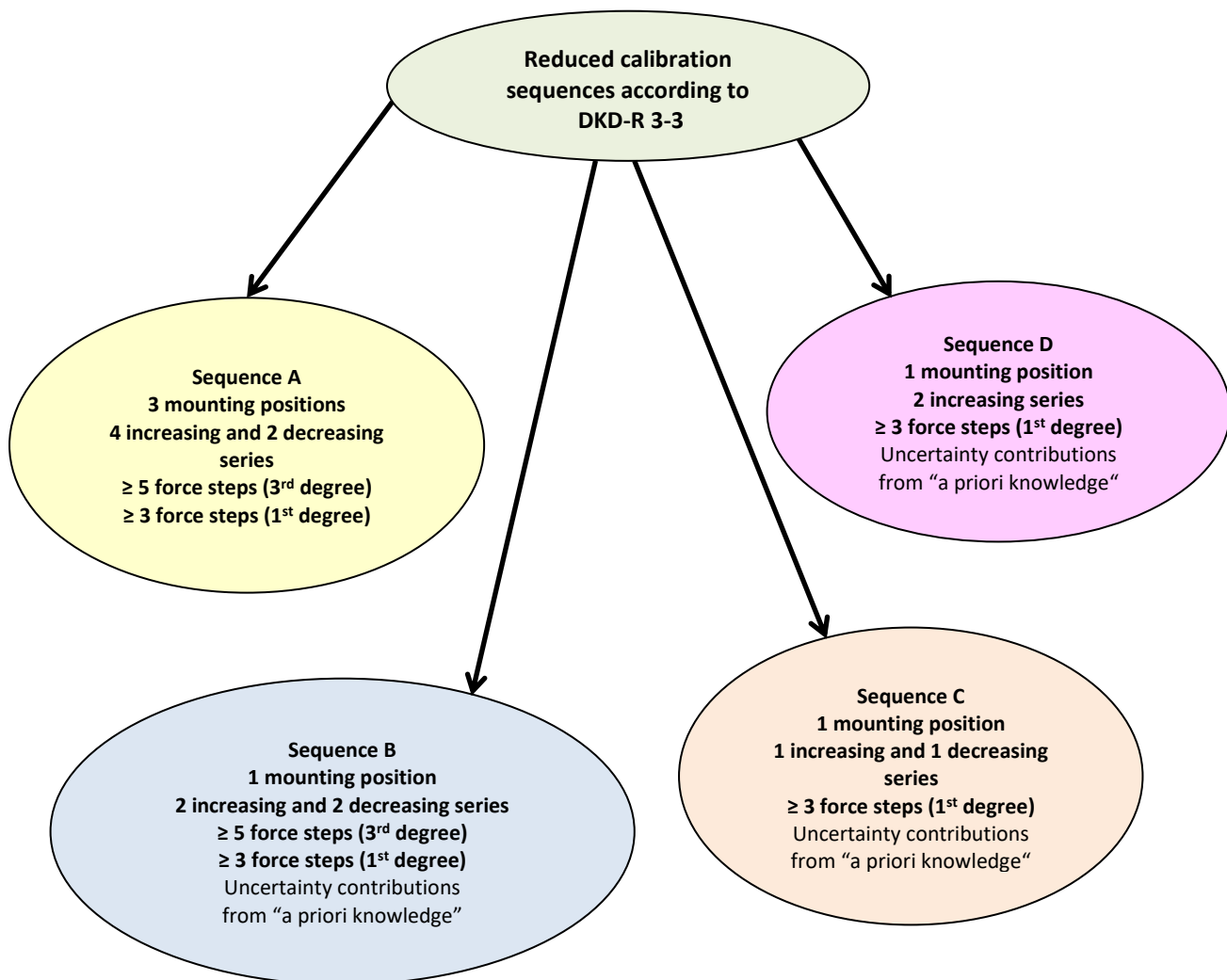
Figure 3: Calibration sequences of DKD-R 3-3 including indication of the number of mounting positions, force steps and the usual degree of the regression function
