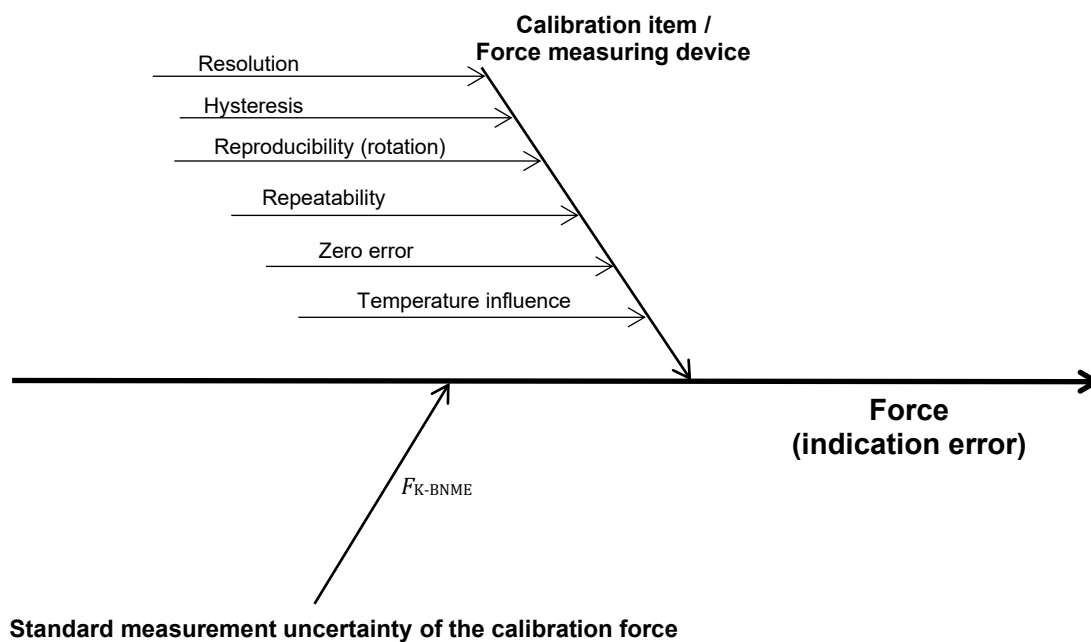
Figure 9: Influence quantities in the determination of the measurement uncertainties associated with the measured values of an indicating measuring device
