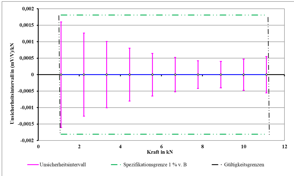
Figure 14: Deviation margin and specification limit
