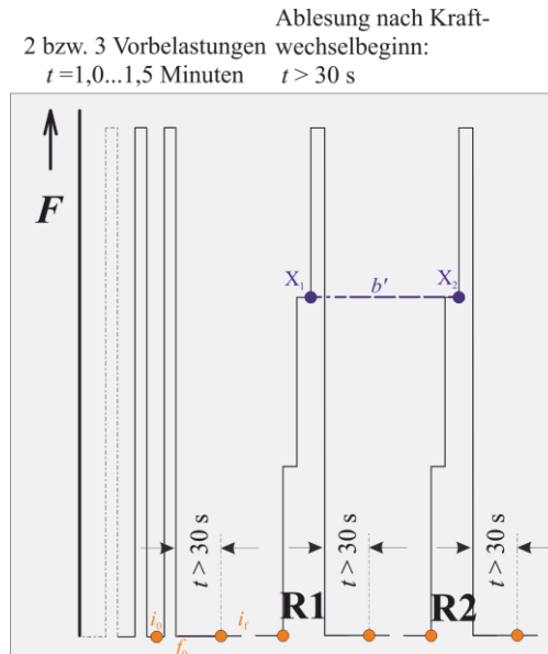
Figure 7: Example calibration sequence D; one mounting position, two measurement series, two increasing loadings, three force steps (2 or 3 preloads, reading after start of force change)
