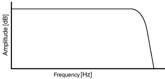
Needed frequency response of a bridge amplifier.
