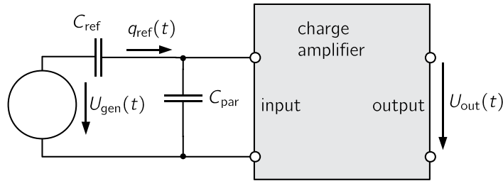
Figure 3: Schematic diagram of a calibration set-up for charge amplifiers.
